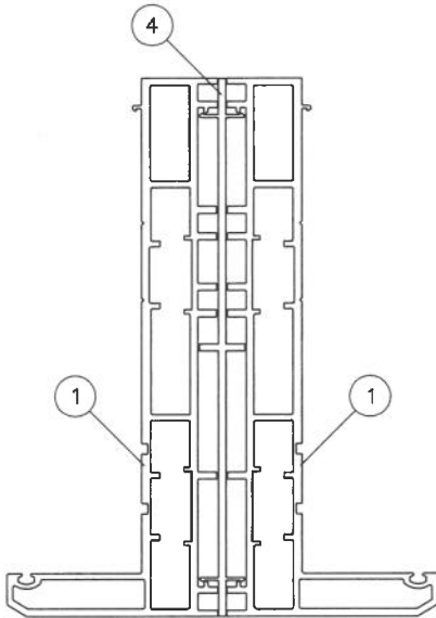
MULLION 'M'
